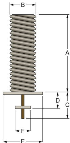
WITH BASE PLATE, SUPPORT PLATE, GROUNDING SPIKE & STEEL CENTERING STRUCTURE
